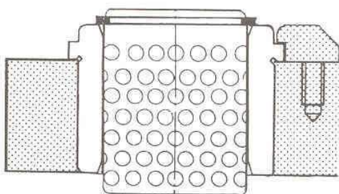
ASSEMBLY OF BUSH AND CAGE
